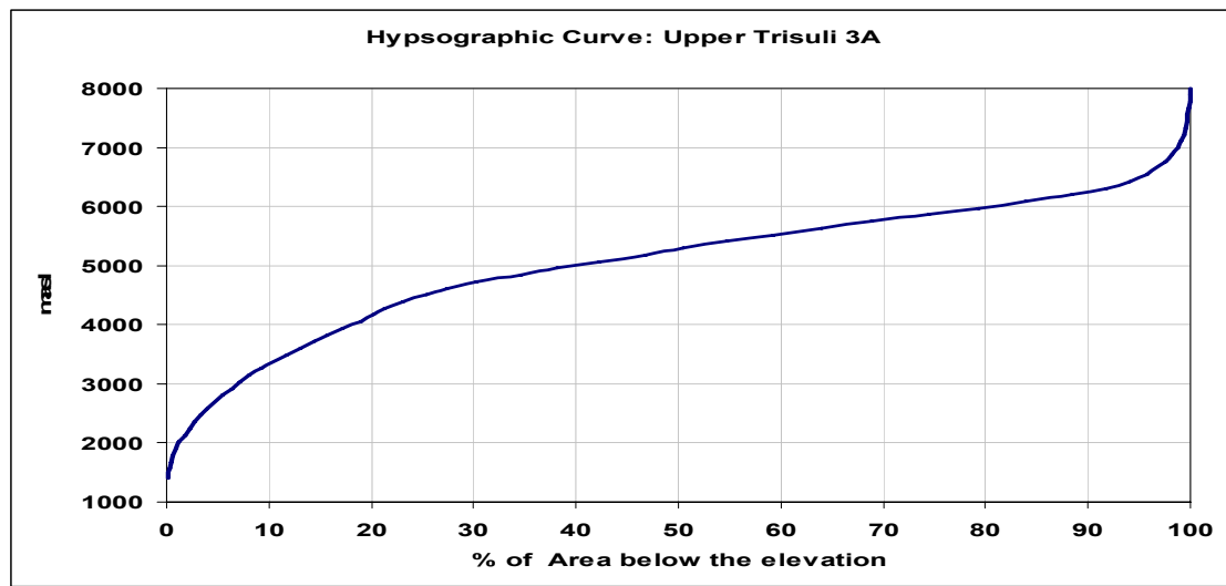
Figure 4 : Hypsographic Curve of Upper Catchment
