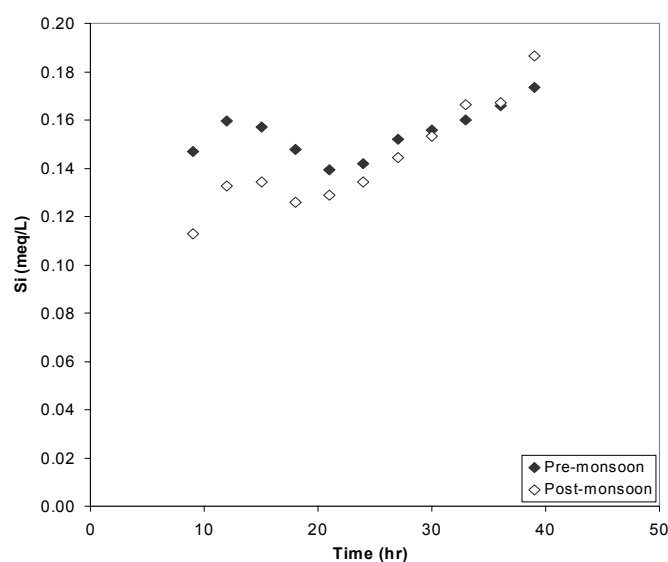
Figure 3. Variation of silicon with time at Lirung outlet during pre-monsoon and post-monsoon season in 1996
