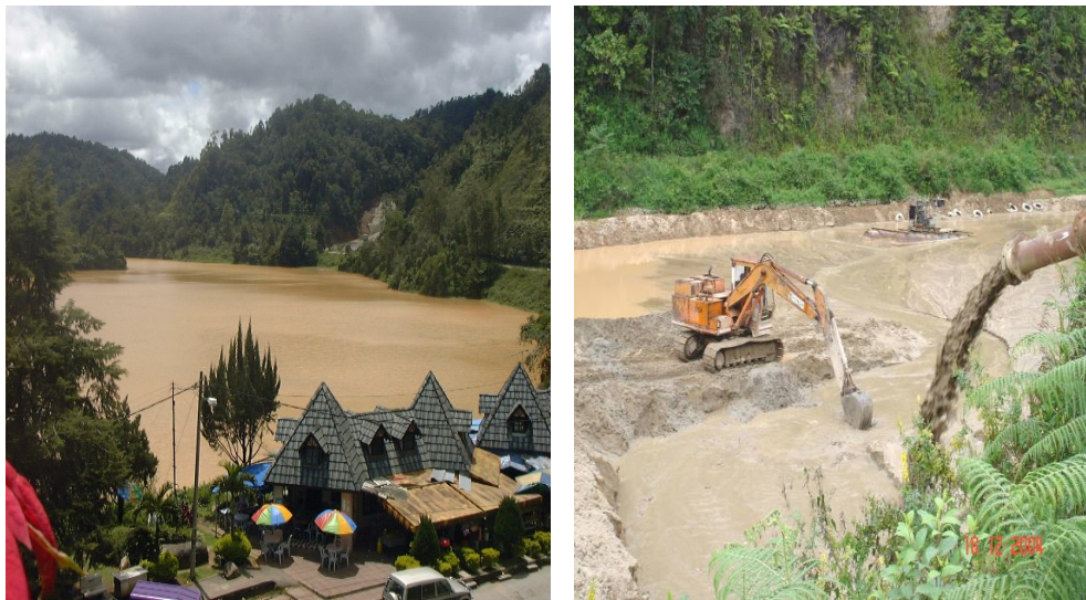
Figure 2 : Sedimentation problems at Abu Bakar Reservoir, Cameron Highlands, Pahang Malaysia (Sinnakaudan, 2006)
