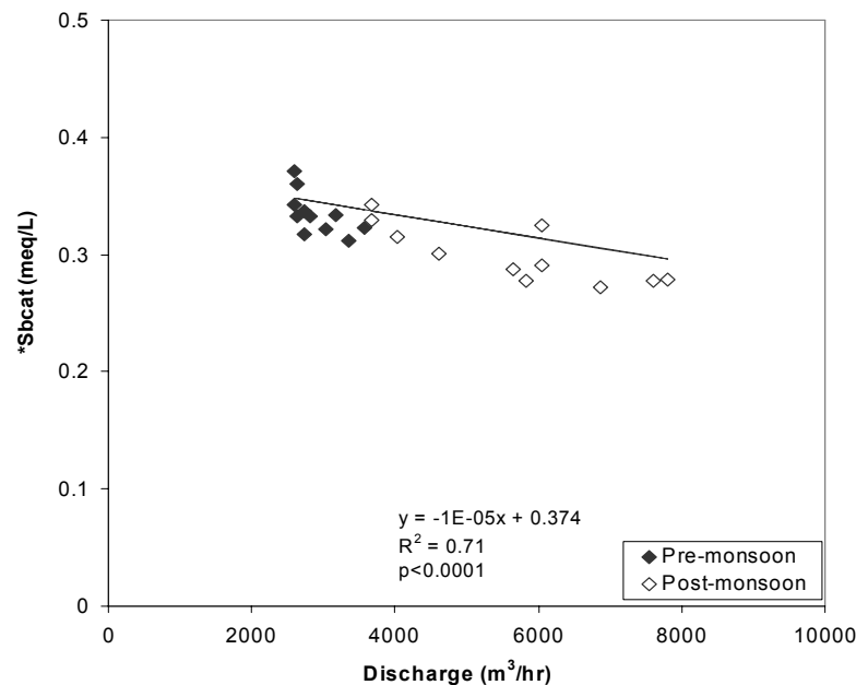
Figure 4. Relationship between sum of base cations after sea-salt correction and discharge at Lirung outlet during pre-monsoon and post-monsoon season in 1996
