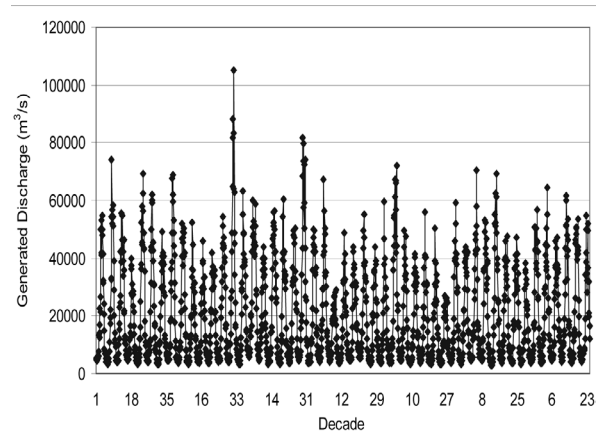
Figure 8: One long time series, out of 200, of generated discharge data
