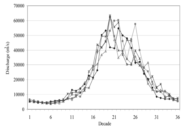
Figure 9: Time series plot of generated data for one year (5 sequences are shown)
