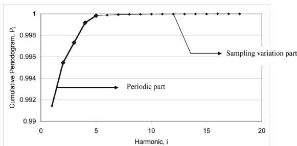
Figure 2: Separation of the cumulative periodogram of decadal means into two parts: periodic (significant) and sampling variation (insignificant)
