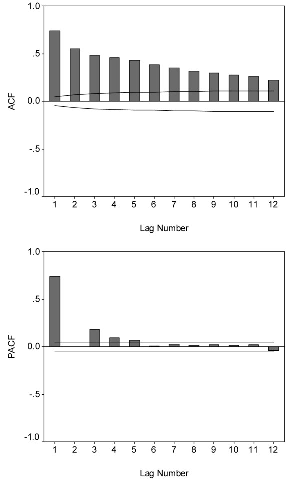
Figure 3: ACF and PACF along with the 95% confidence limits of the deseasonalized, power transformed decadal flow of the Brahmaputra River at Bahadurabad
