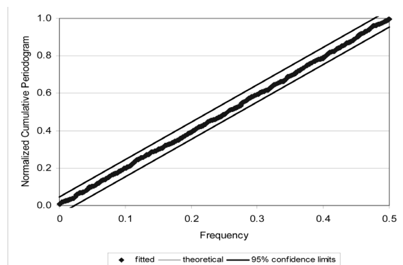
Figure 5: Cumulative periodogram with the 95% large-sample confidence limits for the residuals of the deseasonalized ARMA model
