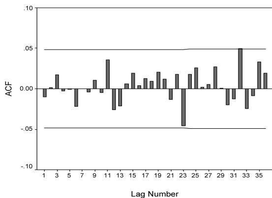
Figure 4: The residual ACF along with the 95% confidence limits of the fitted deseasonalized ARMA model
