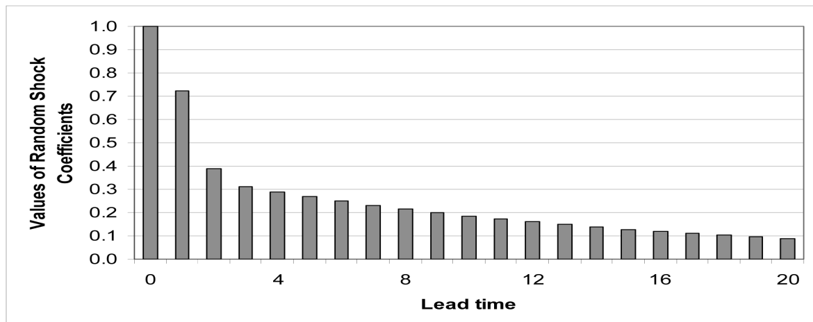
Figure 7: The influence of the current period disturbance on current and future flows
