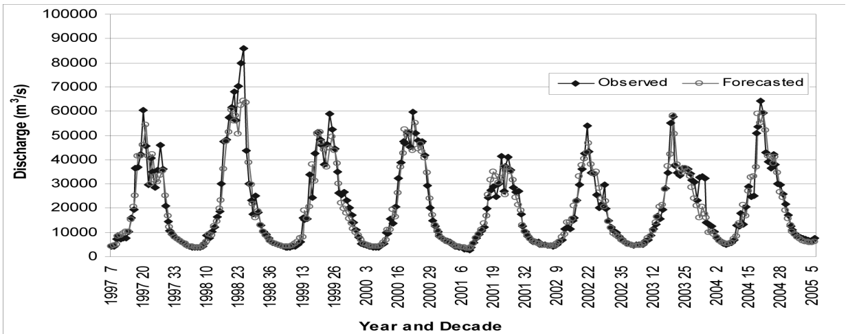
Figure 6: One-step-ahead forecasted flows along with the observed flows from the first decade of March 1997 to the last decade of February 2005
